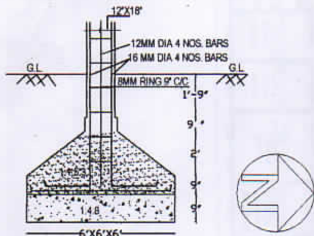
FOUNDATION DETAIL NORTH
