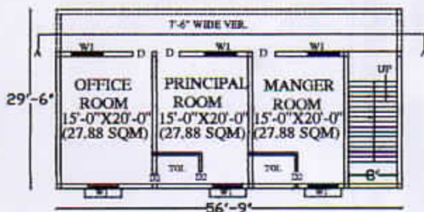
PROP. GROUND FLOOR PLAN
